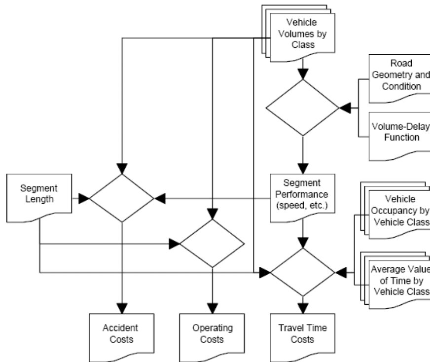
Figure 2-2. Stylized Representation of the User Cost Linkages
